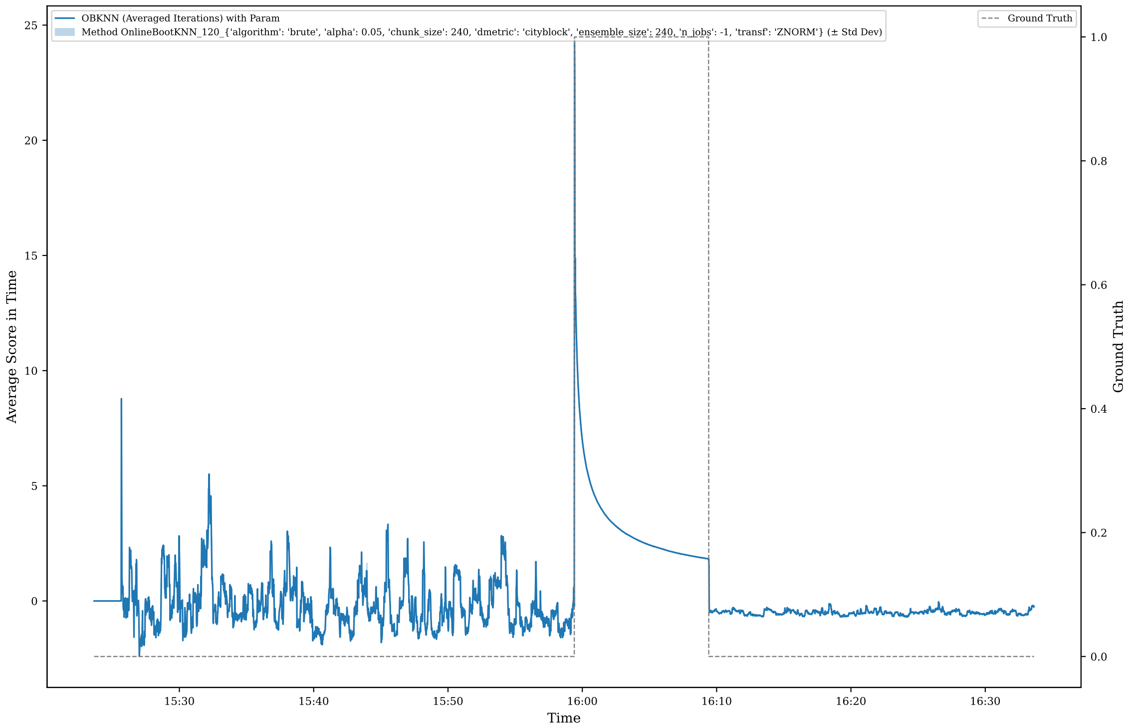
Method OBKNN Score for Scenario A3
